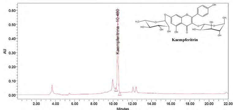
Fig. 1. HPLC elution pattern of kaempferitrin from Justicia spicigera ethanolic extract.
